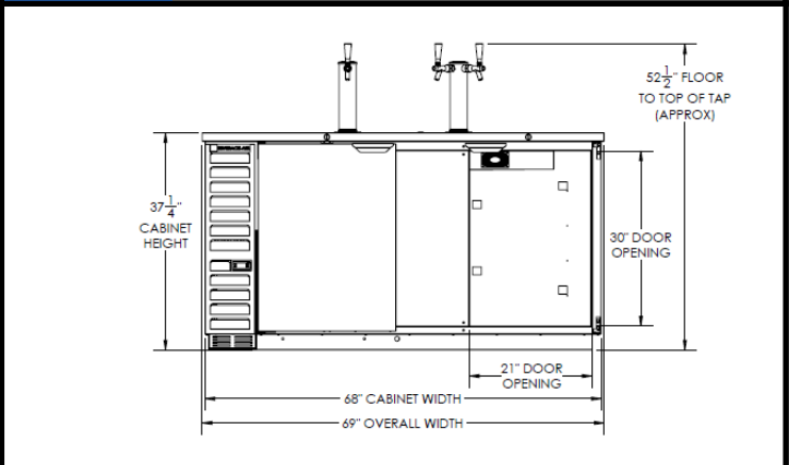
Elevation View
