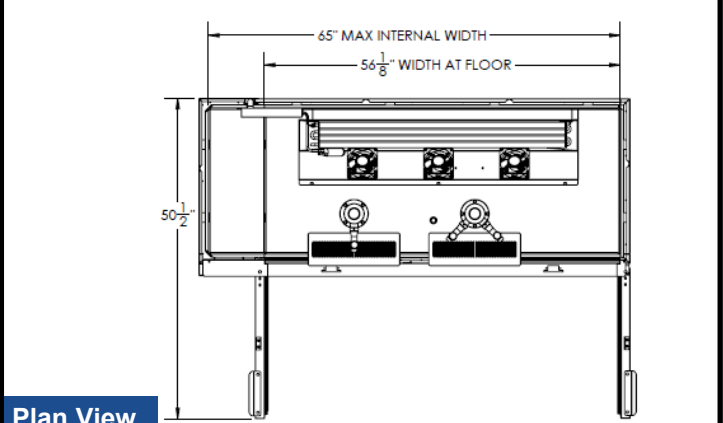
Plan View
